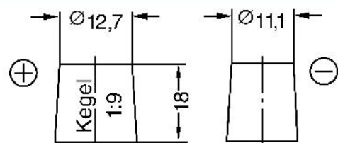
TERMINAL 3
